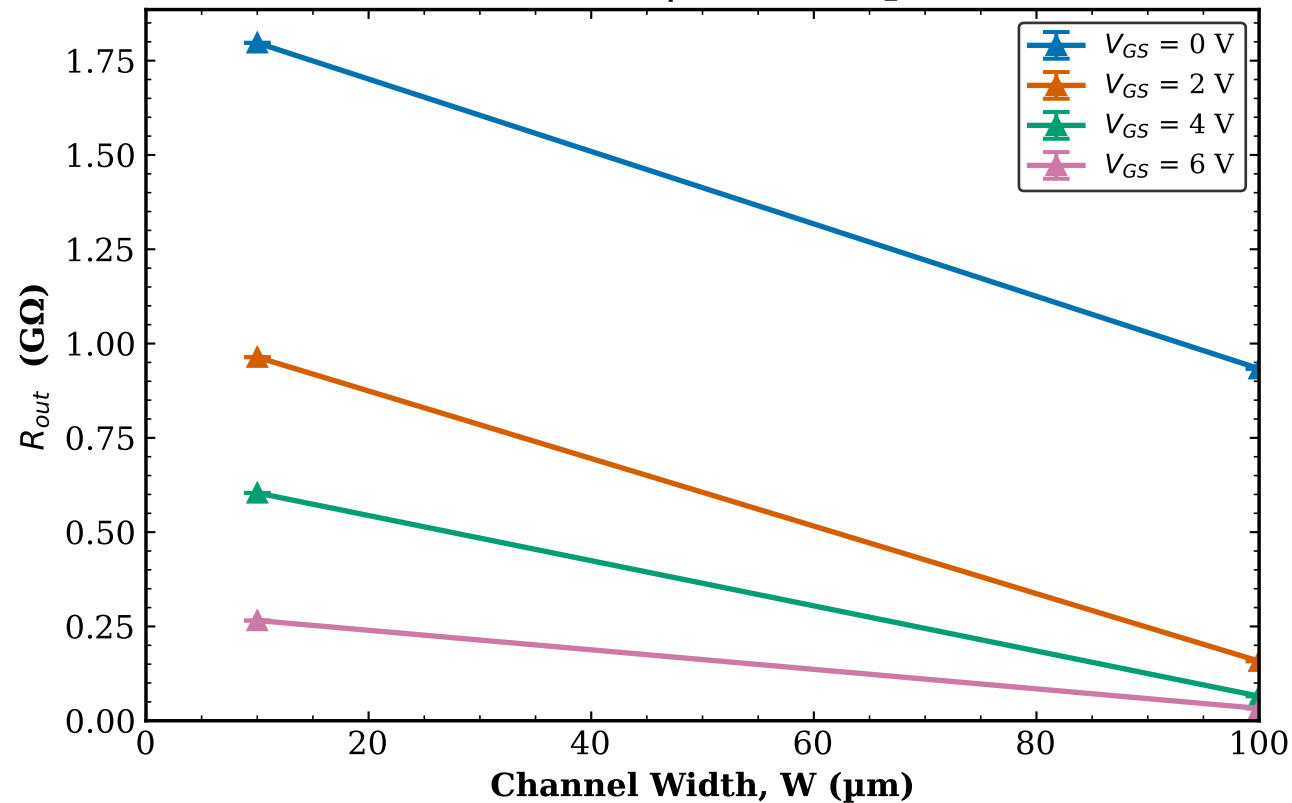
TFT1 Transistor 2 R_{out} vs W | L = 160\text{ }\mu\text{m}
